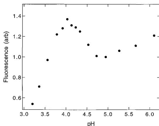
Fig. 1. Fluorescence from apomyoglobin in 10 mM acetate at 50^\circ\text{C} as a function of pH. Excitation was at 278 nm and emission was monitored at 320 nm. The peak around pH 4 is characteristic of the ‘molten globule’ equilibrium intermediate state.
